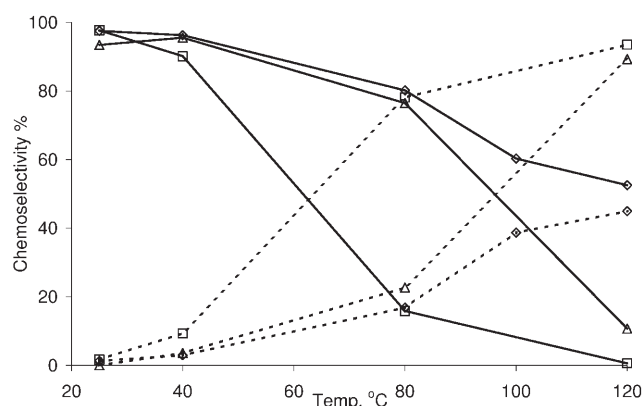
Figure 3. Comparison of overall chemoselectivity towards chlorinated products 5a–d , —, and dechlorinated products 6–9 , ....., in the presence and absence of SCFs. Traces are labelled: \square performed in THF only; \triangle \text{scCO}_2 + THF *; \diamond \text{scC}_3\text{H}_8 + THF **. Reaction conditions: \text{H}_2 P=1 bar; 0.05 g of 5% Pd/CaCO 3 cat.; 4.5 mL of 0.05 M solution in THF; reaction time = 40 min; * \text{CO}_2 P=175 bar; ** \text{C}_3\text{H}_8 P=175 bar.
