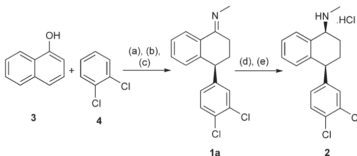
Scheme 1. Current Pfizer synthesis to make Zoloft®. (a) \text{AlCl}_3 ; (b) simulated moving bed chromatography (SMB); (c) \text{MeNH}_2 , \text{EtOH} ; (d) \text{Pd/CaCO}_3 , \text{H}_2 , \text{EtOH} ; (e) \text{HCl} , \text{EtOH} . [14]
